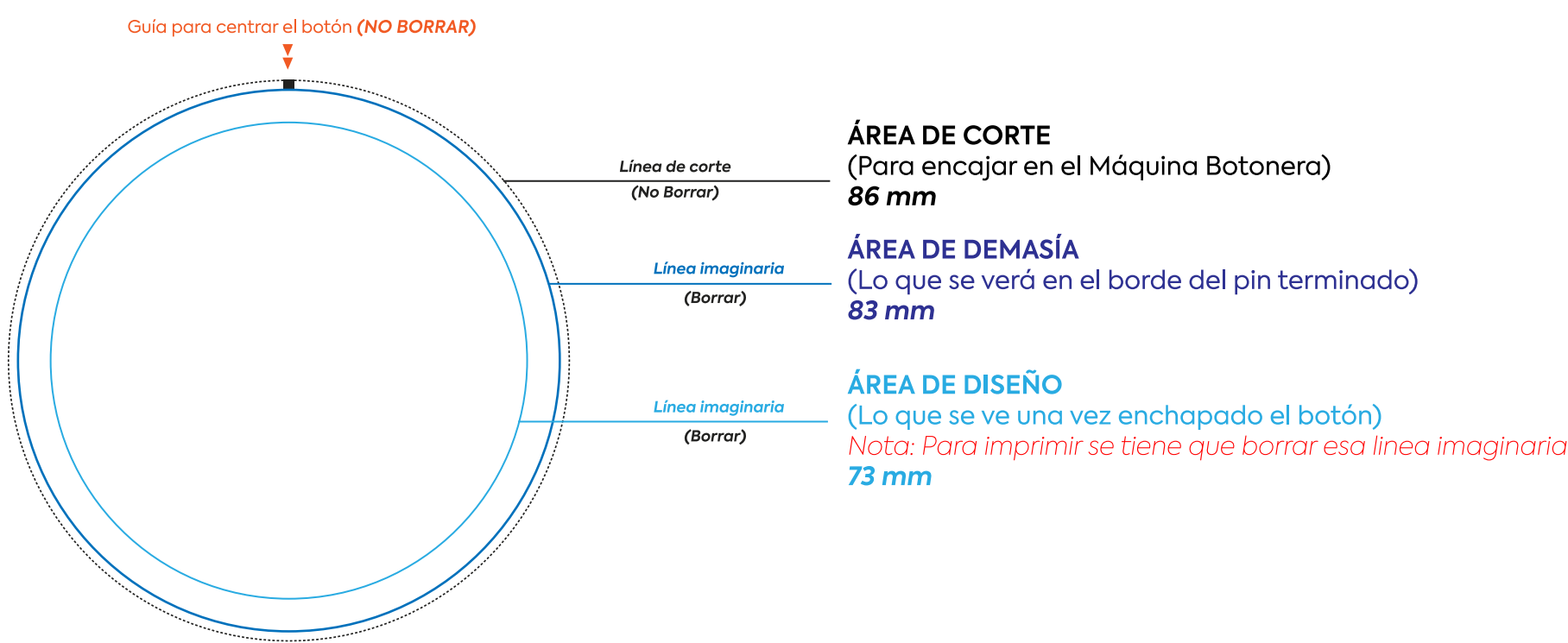
Pin 75mm
